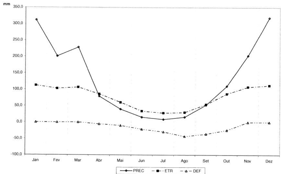
Figure 13 – Hydric Balance (1981-2003). Source: SILVA and ASSUNÇÃO, 2004.
