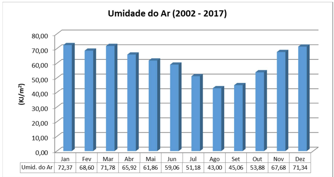
Figure 8 – Air moisture at Uberlândia station (2002-2017). Source: INMET, 2018.
