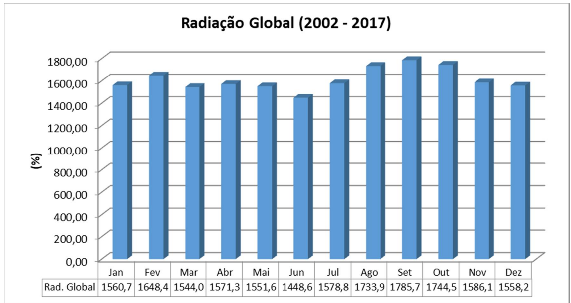
Figure 9 – Global solar radiation at Uberlândia station (2002-2017). Source: INMET, 2018.
