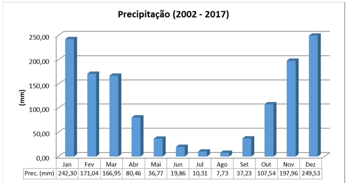
Figure 6 – Rainfall precipitation at Uberlândia station (2002-2017). Source: INMET, 2018.
