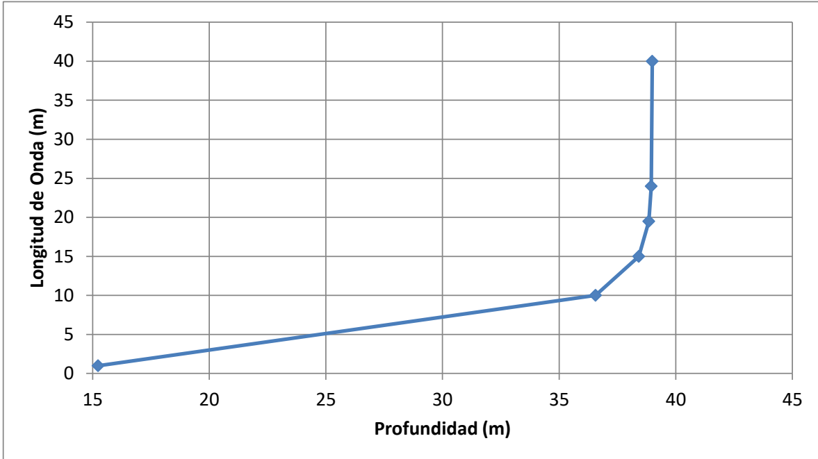
Figure No. 5.144 Wavelength for different depths, for the initial condition of the landfill. Source: Aqua & Terra Consultores Asociados S.A.S, 2013
