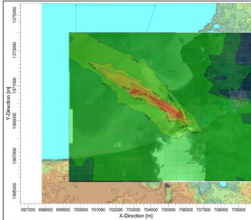
Figure No. 5.235 Sulfur Dioxide modeling result, SO 2 in the study area Source: AG Consultores Ambientales S.A.S., 2015
