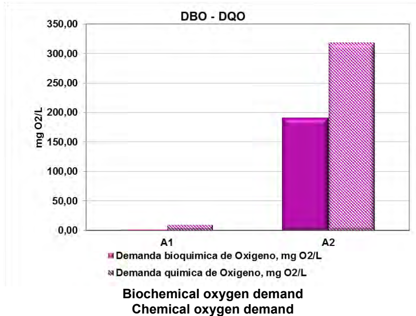
Figure 5.48 BOD5-COD– surface water Source: Aqua & Terra Consultores Asociados S.A.S., 2015 with results from SGS S.A.S, 2015
