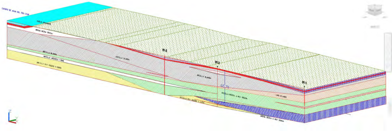
Figure 5.105. Block Diagram in Zone of Influence II Source: Aqua & Terra Consultores Asociados S.A.S. (2015)
