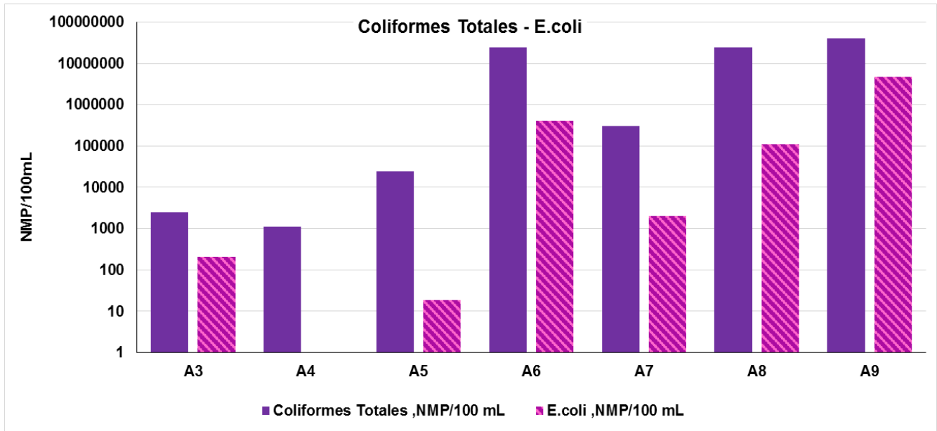
Figure No. 5.166 Behavior Total coliforms and E coli – Marine water Source: Aqua & Terra Consultores Asociados S.A.S., 2015 with results from SGS S.A.S, 2015
