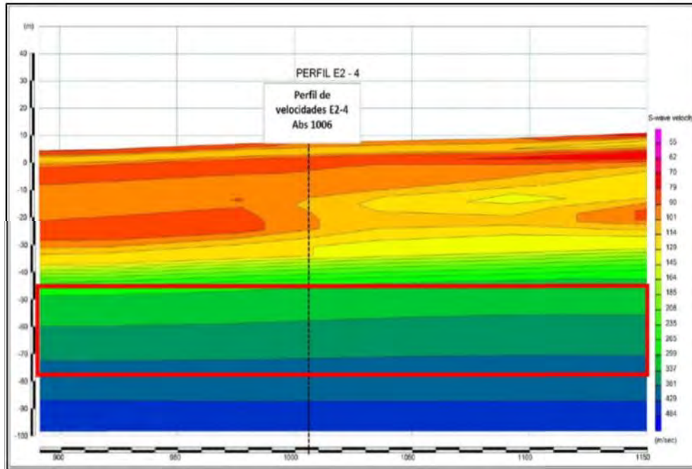
Figure 5.92. ReMI shear wave velocity cross-section (Profile E2-4) Source: ULLOA Y DIEZ LTDA, in PIO S.A.S (2015) 161
