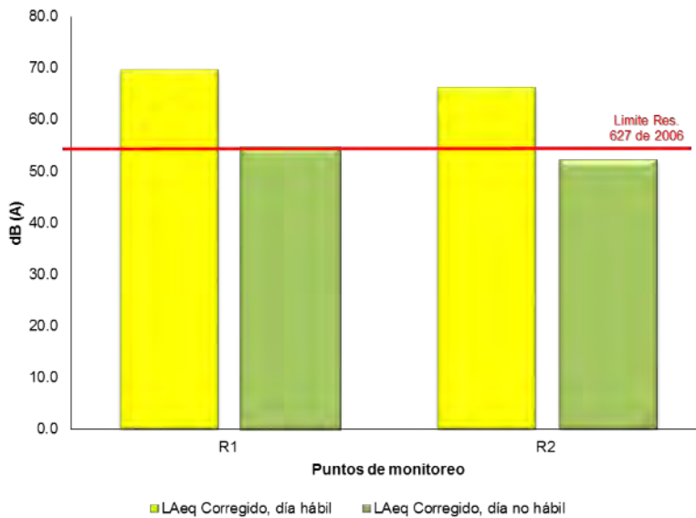
Monitoring Points----Corrected LAeq(working day)-- Corrected LAeq(non-working day) Figure No. 5.239 Environmental noise at night time, monitoring points R1 and R2 Source: SGS COLOMBIA S.A.S., Julio 2015
