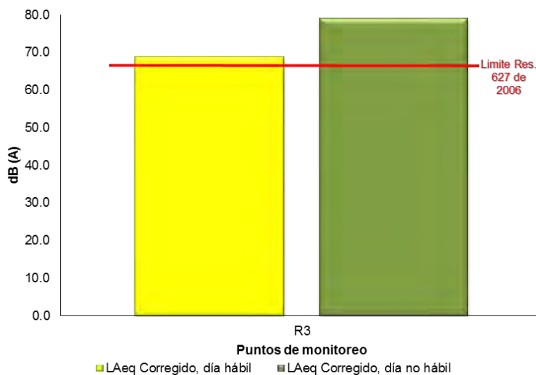
Monitoring Points----Corrected LAeq(working day)-- Corrected LAeq(non-working day)
