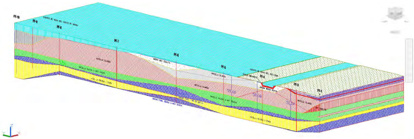
Figure 5.104. Block Diagram in Zone of Influence I Source: Aqua & Terra Consultores Asociados S.A.S. (2015)
