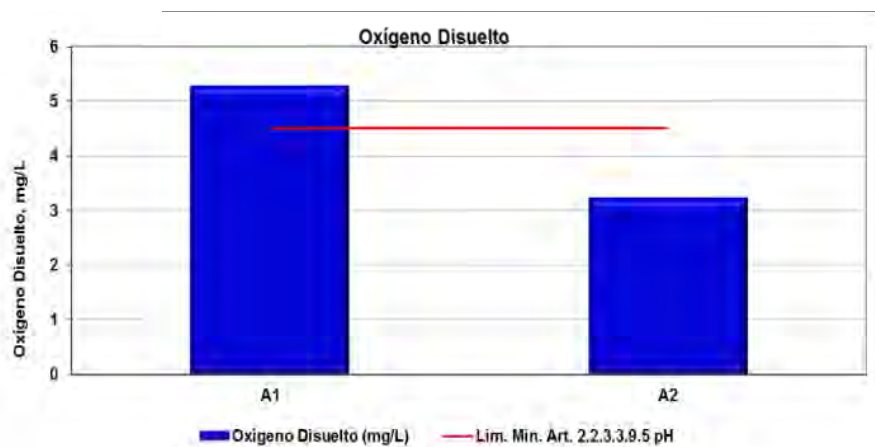
Figure 5.40 Dissolved oxygen results – surface water Source: Aqua & Terra Consultores Asociados S.A.S. (2015) with results from SGS S.A.S (2015)
