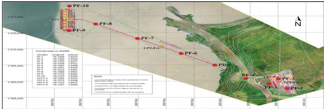
Figure 5.101. Location of ground hydrogeological profiles Source: EDIFICA COLOMBIA LTDA, in PIO S.A.S (2015) 172
