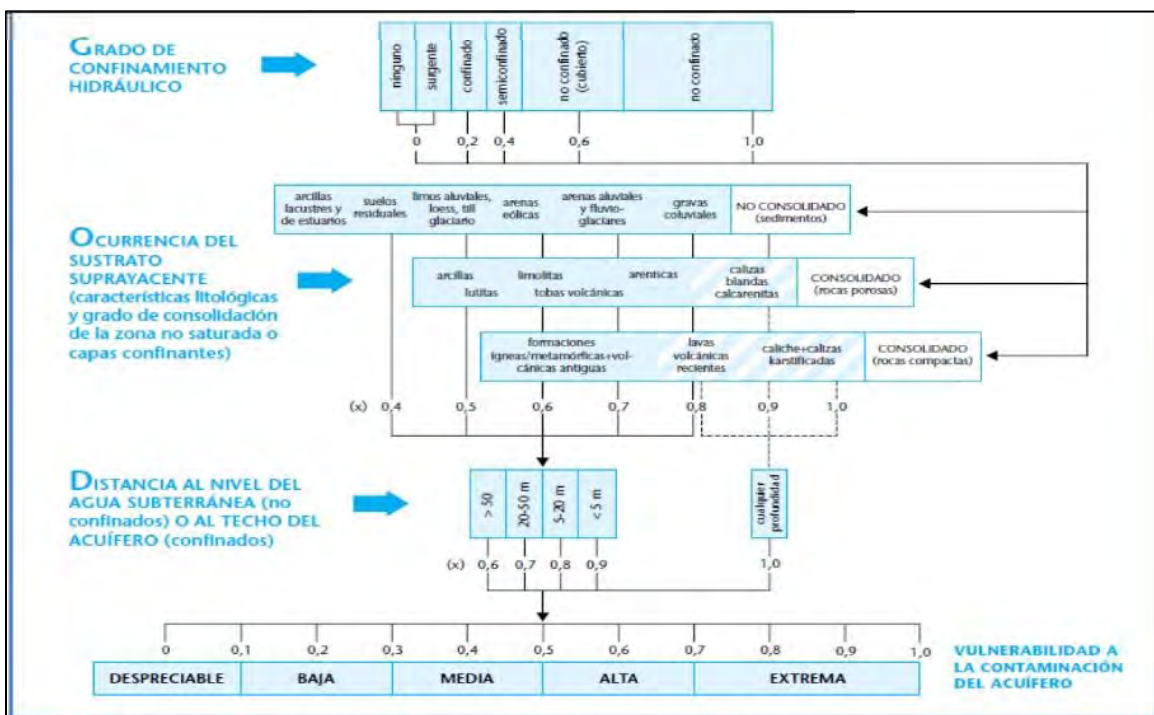
Figure 5.106. Diagram of the GOD method for evaluating intrinsic vulnerability. Source: Environment, Housing and Territorial Development Ministry (2010) 175
