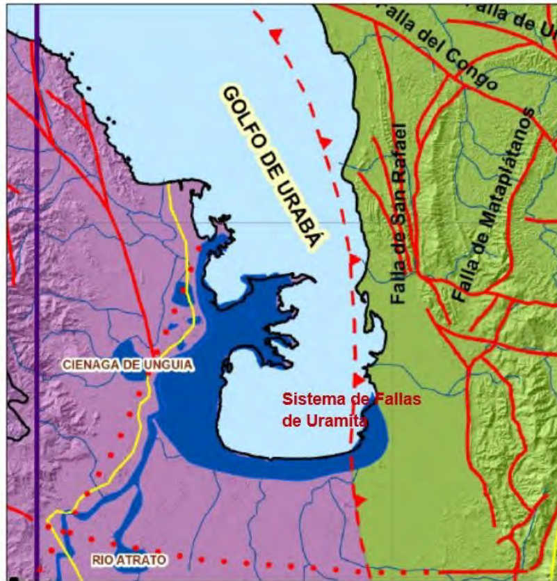
Figure 5.76 Tectonic diagram of the Urabá region, showing the Uramita Fault. Source: INGEOMINAS 1999 and 2005, in PIO S.A.S, 2015 134
