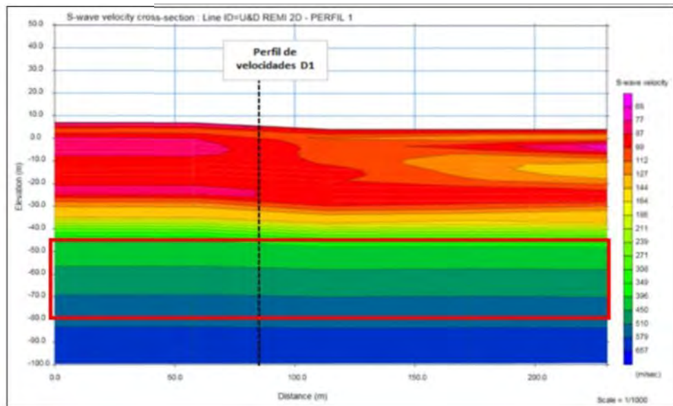
Figure 5.87 ReMI shear wave velocity cross-section (Profile D1) Source: ULLOA Y DIEZ LTDA , in PIO S.A.S , 2015 156
