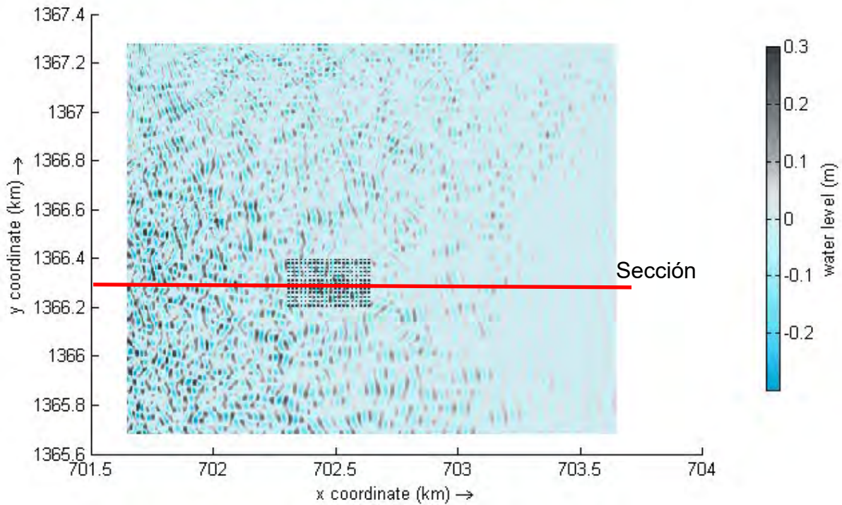
Figure No. 5.138. Distribution of the waves with piles and bottom changes by dredging. Source: Aqua & Terra Consultores
