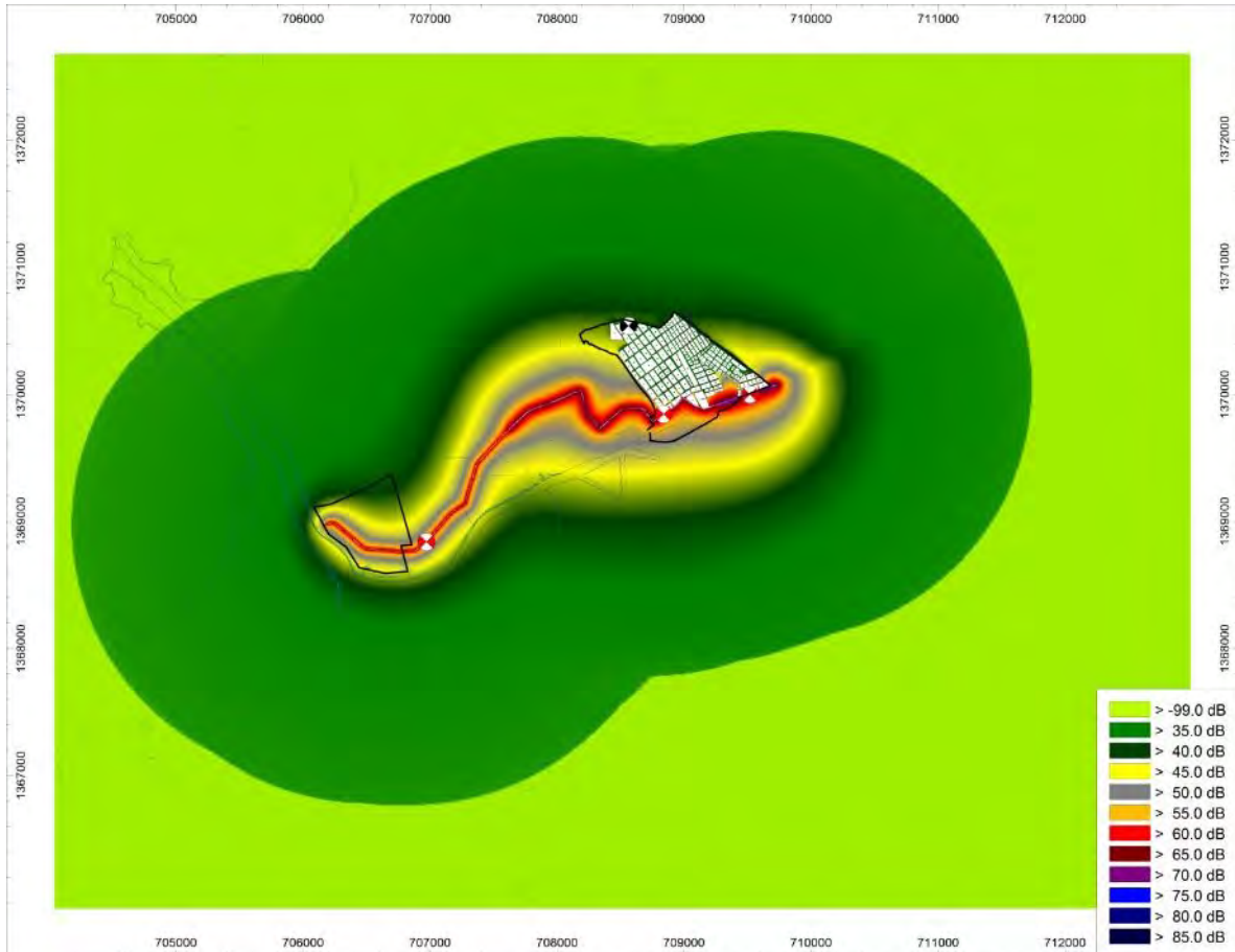
Figure No. 5.251 Noise Map Generated by CadnaA - Raster Format. Scenario I. CadnaA. Source: SGS COLOMBIA S.A, 2015 with CadnaA Software, 2015
