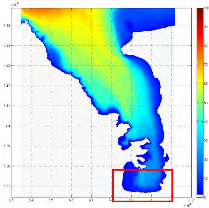
Figure No. 5.123 b) a) General Mesh and b) Detail used to reach the study area with model SWAN. Source: Aqua & Terra Consultores Asociados S.A.S, 2015
