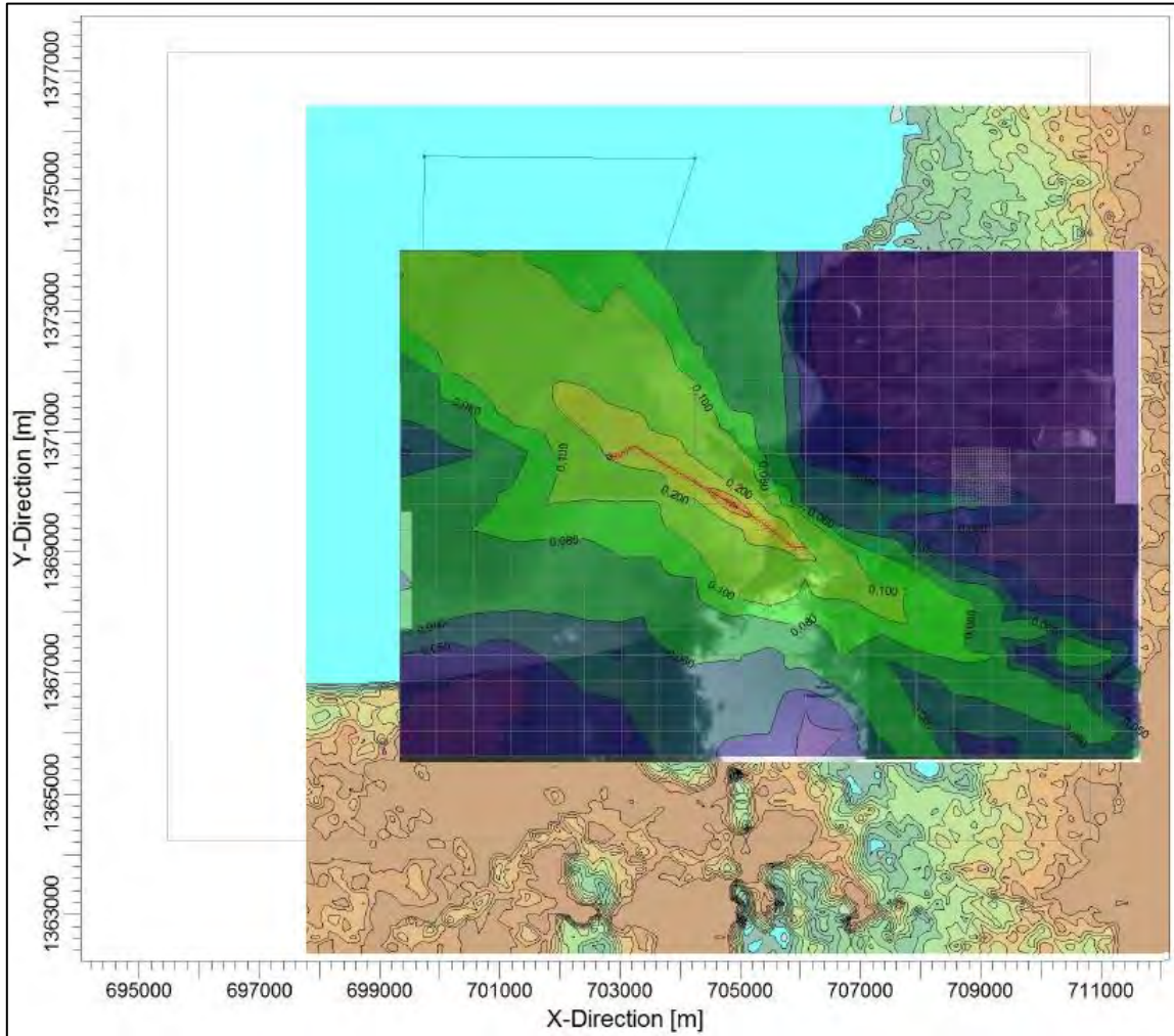
Figure No. 5.236 Carbon Monoxide modeling result, CO in the study area. Source: AG Consultores Ambientales S.A.S., 2015
