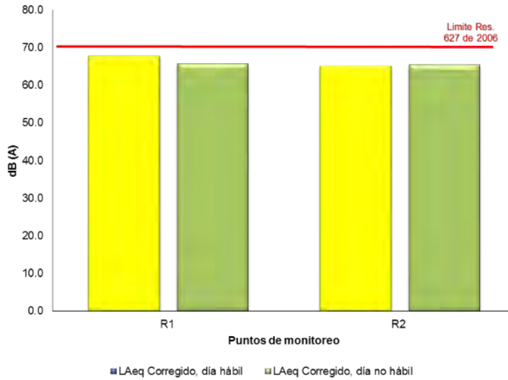
Monitoring Points----Corrected LAeq(working day)-- Corrected LAeq(non-working day) Figure No. 5.238 Environmental noise during the day, monitoring points R1 and R2 Source: SGS COLOMBIA S.A.S., July 2015
