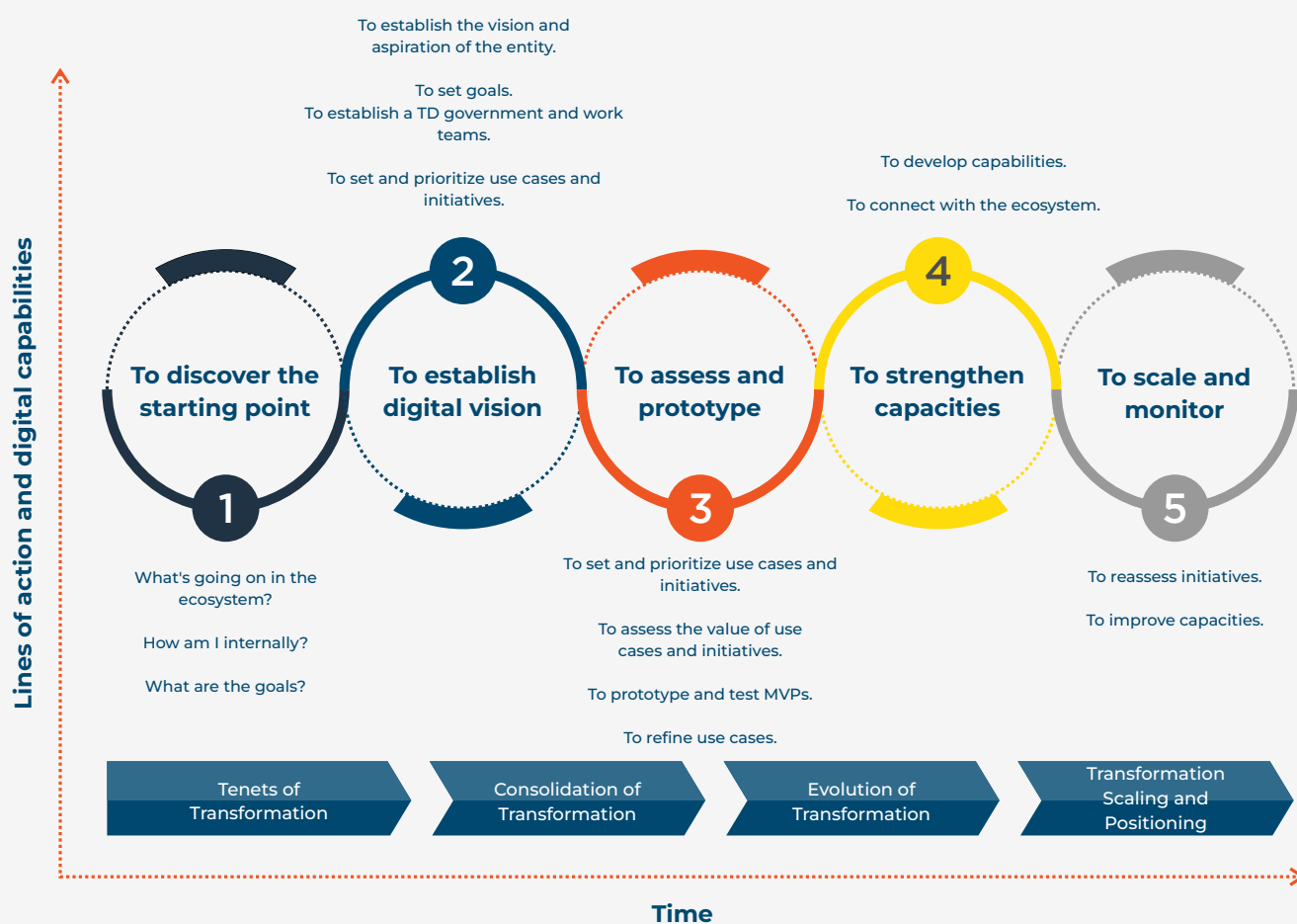
Figure 40: Roadmap Stages
